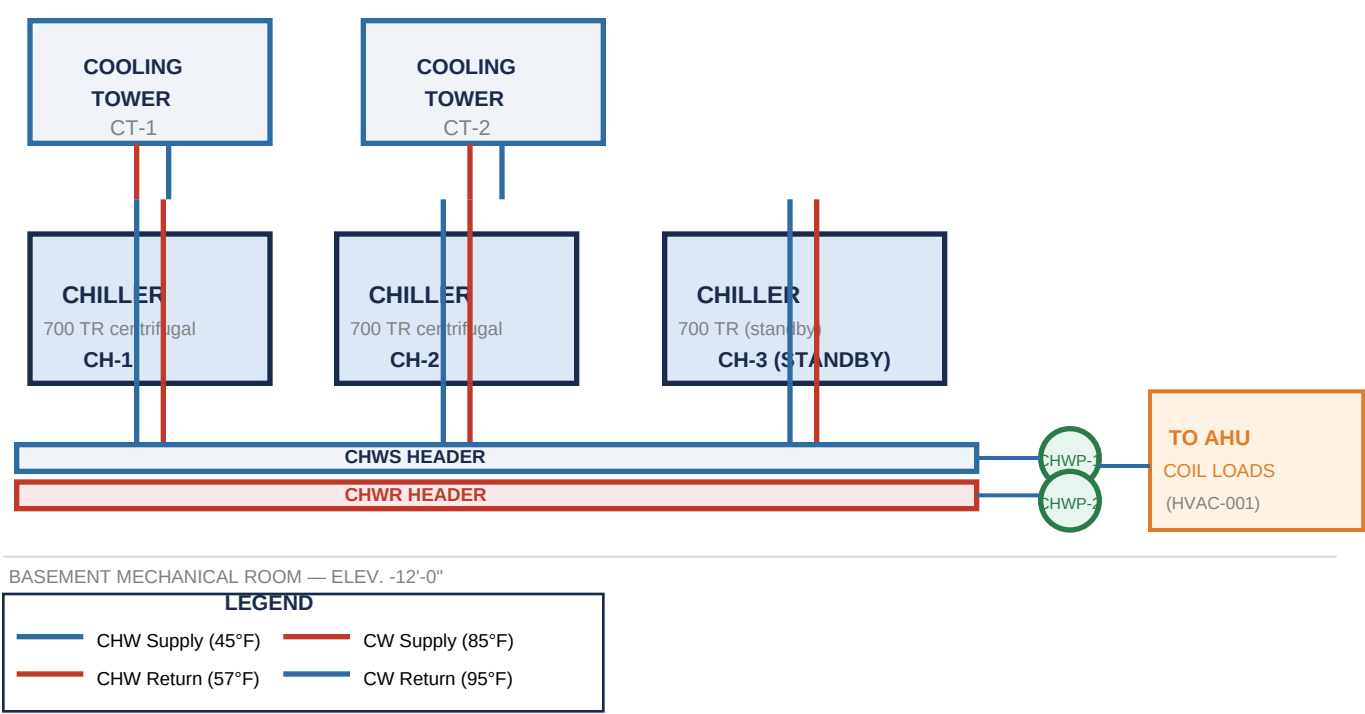
Figure 4 — Chilled Water Plant Piping Schematic (Not to Scale)
